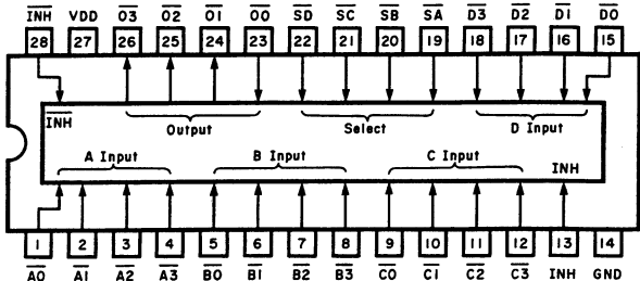
Fig. 8.1.7 Input Port Expander LC7800
