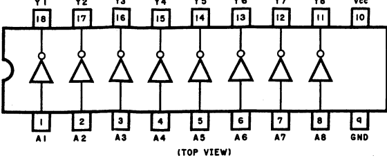
Fig. 8.1.9 FL Display Tube Driver LB1240
