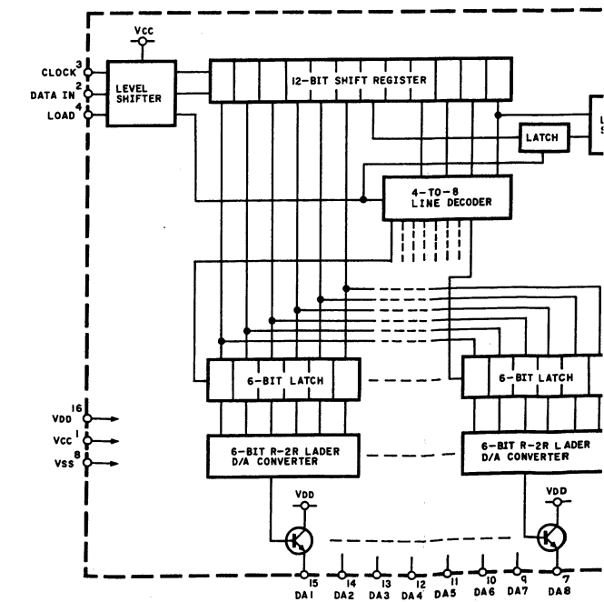
Fig. 8.1.16 μPD6326C-028
