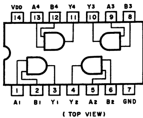
Fig. 8.1.2 AND Gate C-MOS IC \mu PD4081BC
