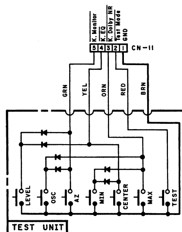
Fig. 5.3 Circuit Diagram of Test Unit
