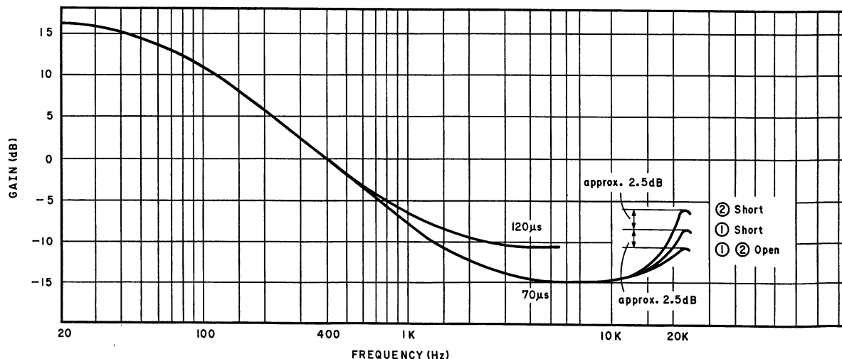
Fig. 5.5 Playback Eq. Curve
