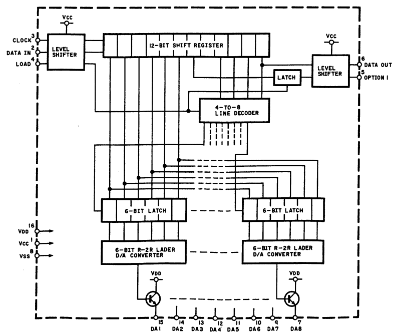
Fig. 8.1.16 μPD6326C-028
