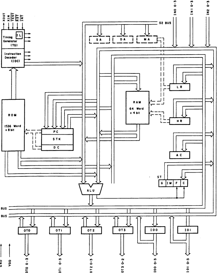
Fig. 8.1.11 4-Bit Micro-processor TMP4315BP-1814
